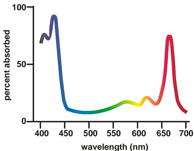
Absorption spectrum of chlorophyll a .
